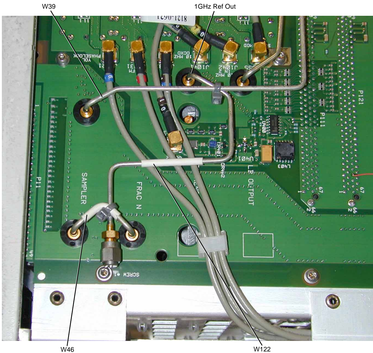
Figure 5 W122 Installation
